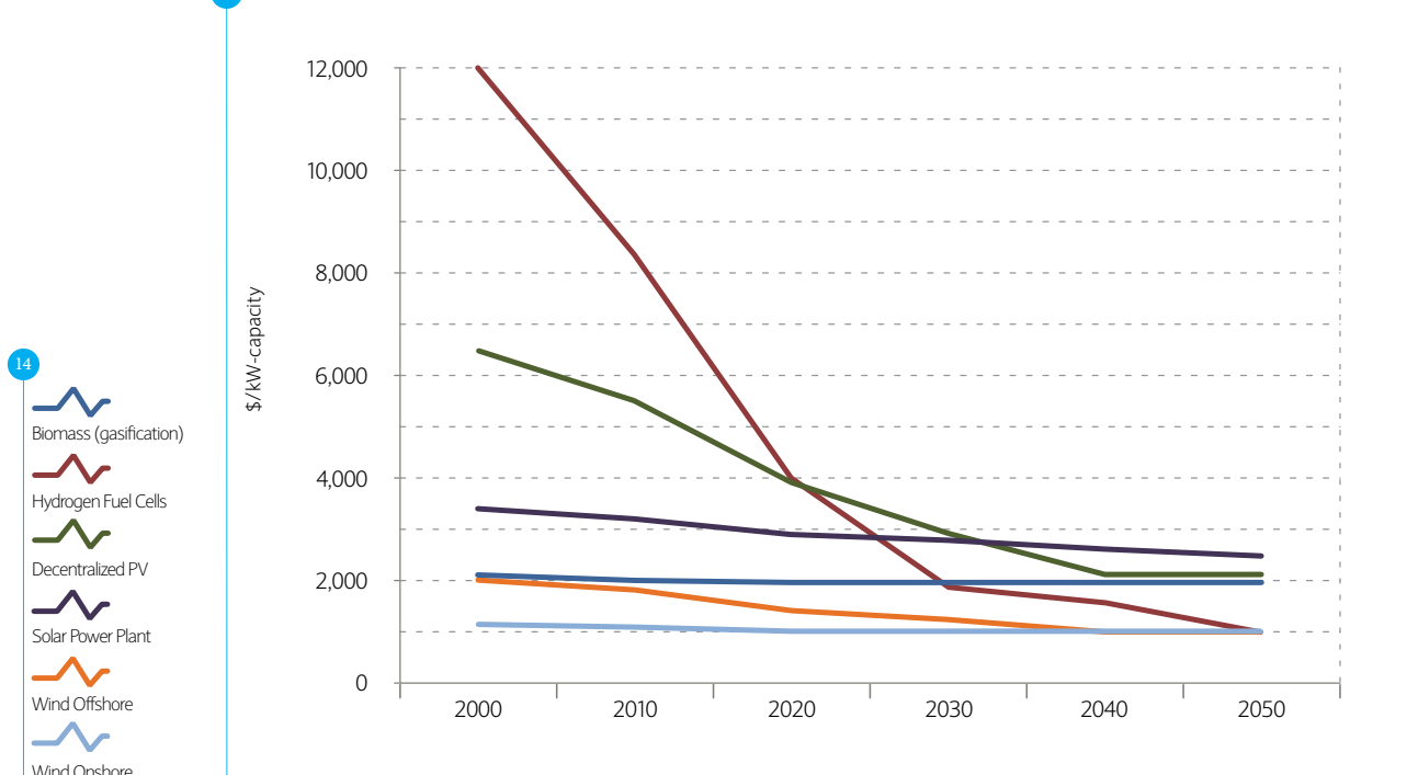
14 COST-INTENSITY OF ALTERNATIVE POWER PRODUCTION
